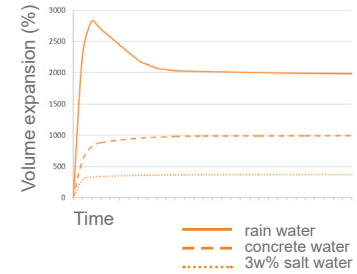
SEALING INSERT superswell version 4 mm
