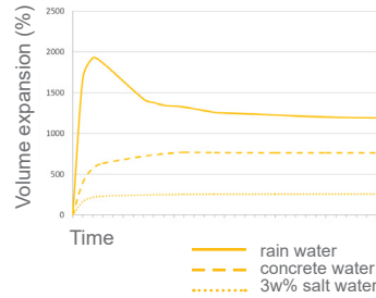
SEALING INSERT salt version 4 mm
